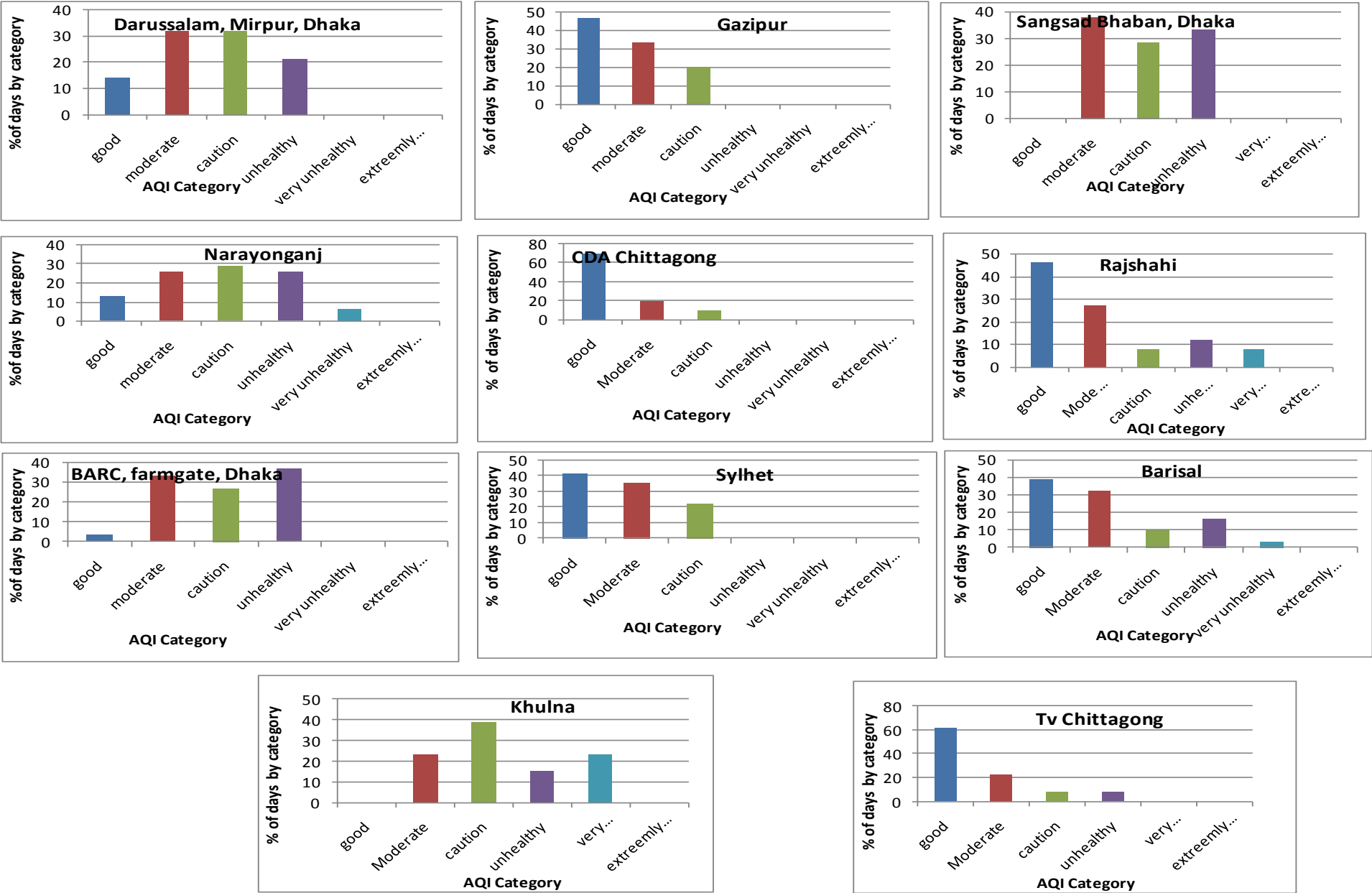
Figure 5: Monthly Summary of AQI for month of October, 2017
