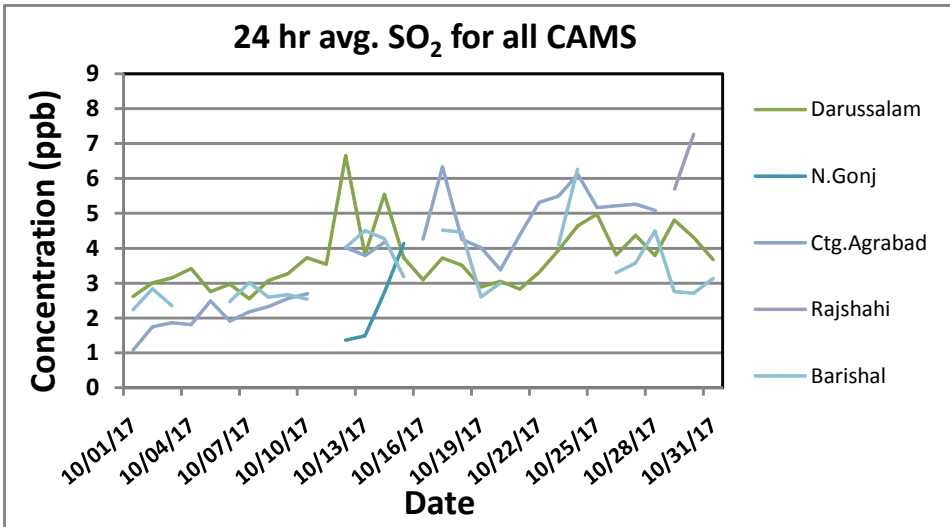
FIGURE 3: TIME SERIES OF ALL PARAMETERS (SO 2 , NO x AND O 3 ) MEASURED IN ALL CAMS DURING OCTOBER, 2017
