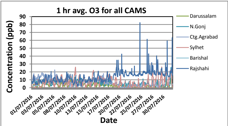
FIGURE 3: TIME SERIES OF ALL PARAMETERS (SO 2 , NO x AND O 3 ) MEASURED IN ALL CAMS DURING JULY, 2016
