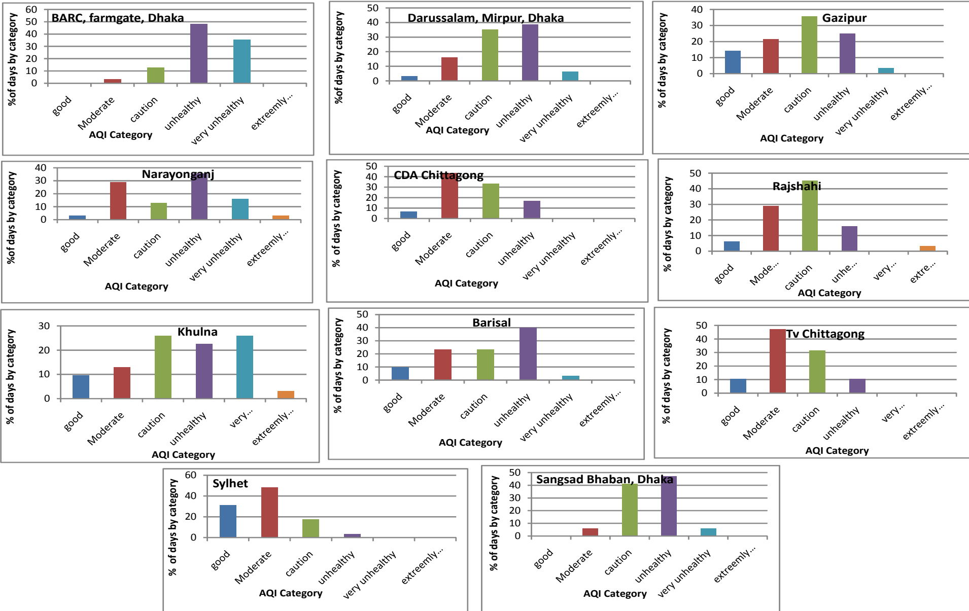
Figure 5: Monthly Summary of AQI for month of October, 2015
