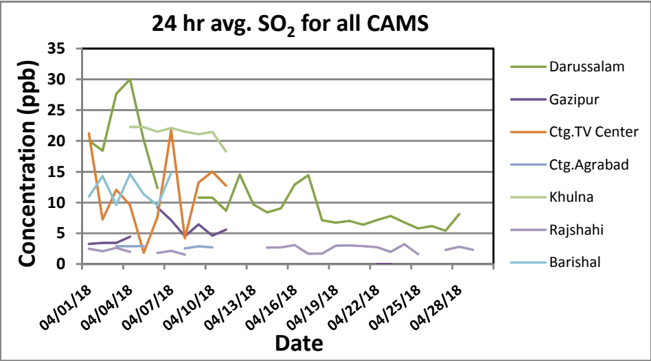
FIGURE 3: TIME SERIES OF ALL PARAMETERS (SO 2 , NO x AND O 3 ) MEASURED IN ALL CAMS DURING APRIL, 2018
