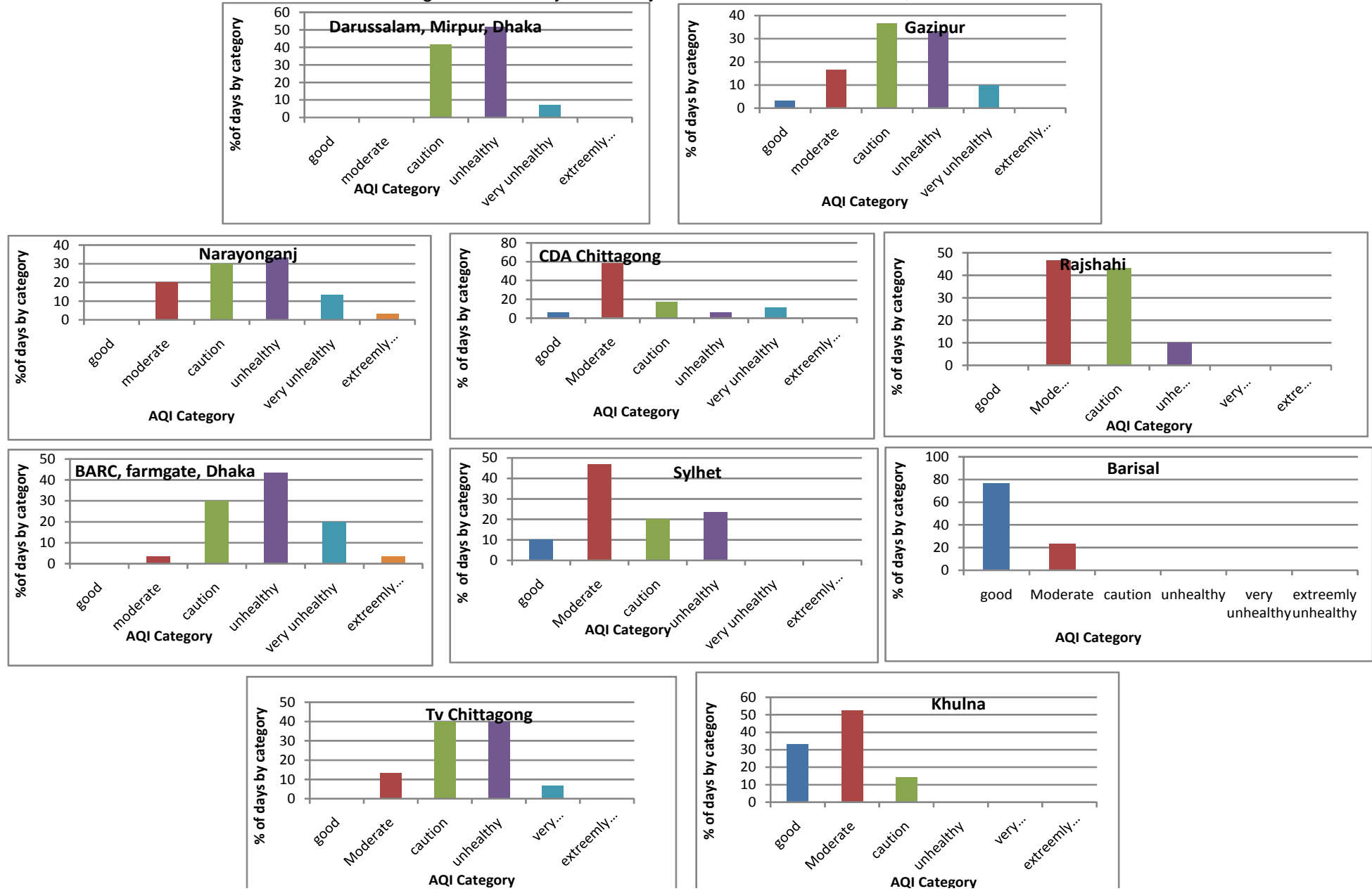
Figure 5: Monthly Summary of AQI for month of APRIL, 2018
