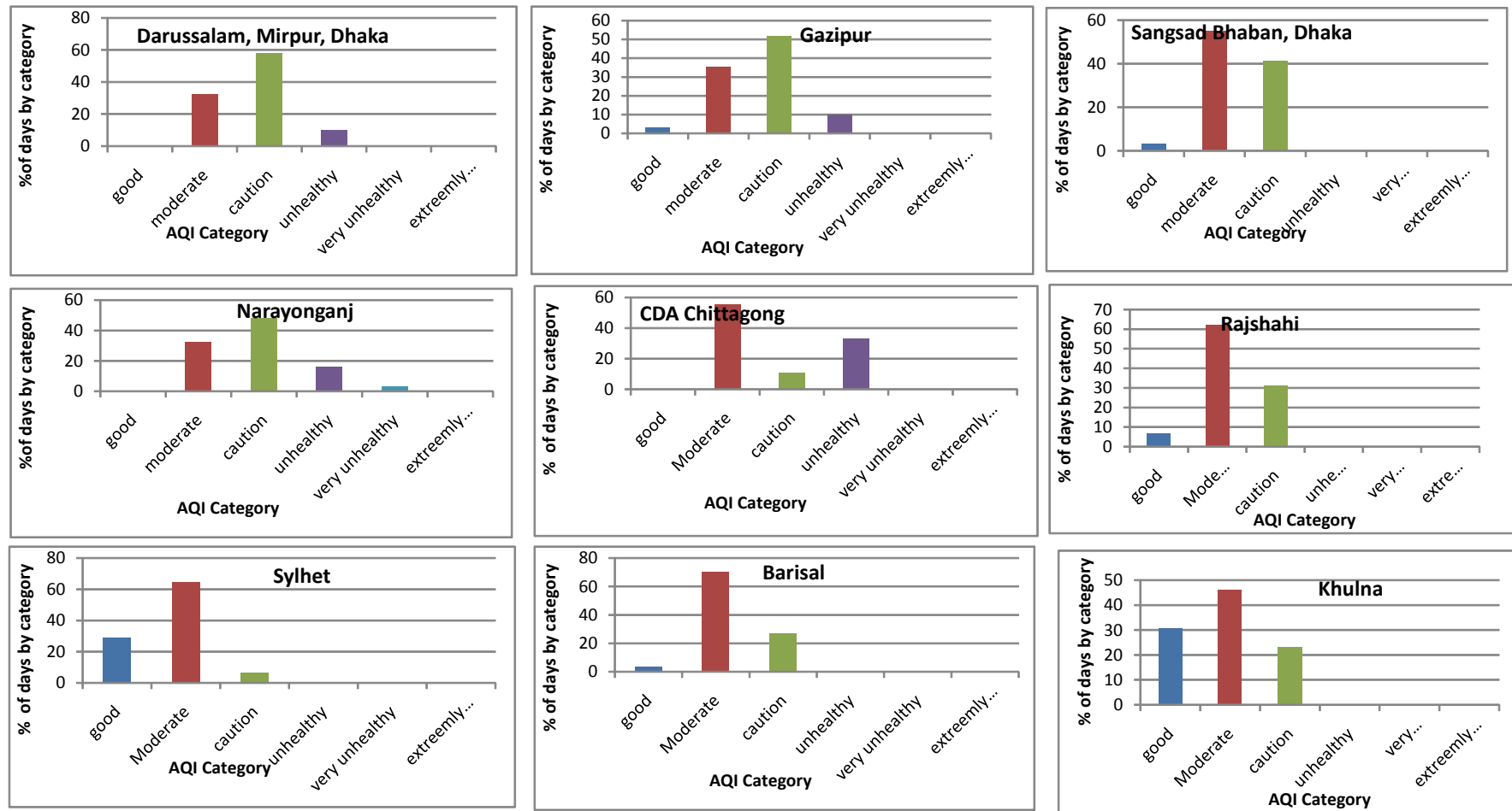
Figure 5: Monthly Summary of AQI for month of MAY, 2017
