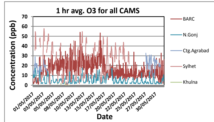
FIGURE 3: TIME SERIES OF ALL PARAMETERS (SO 2 , NO x AND O 3 ) MEASURED IN ALL CAMS DURING MAY, 2017
