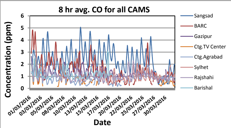
Figure 4: TIME SERIES OF ALL PARAMETERS (CO, PM10 AND PM2.5) MEASURED IN CAMS DURING MARCH, 2016
