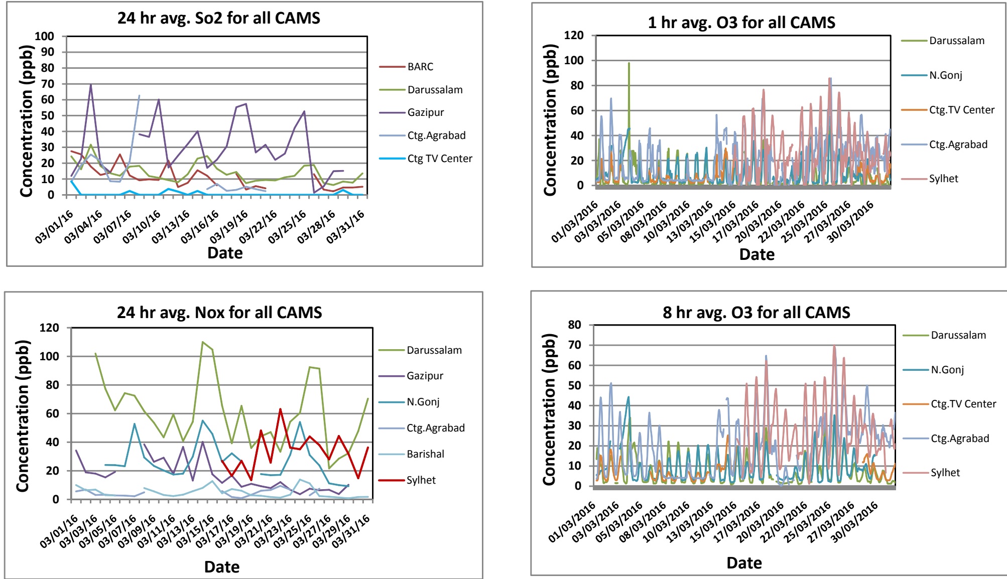
FIGURE 3: TIME SERIES OF ALL PARAMETERS (SO 2 , NO x AND O 3 ) MEASURED IN ALL CAMS DURING MARCH, 2016
