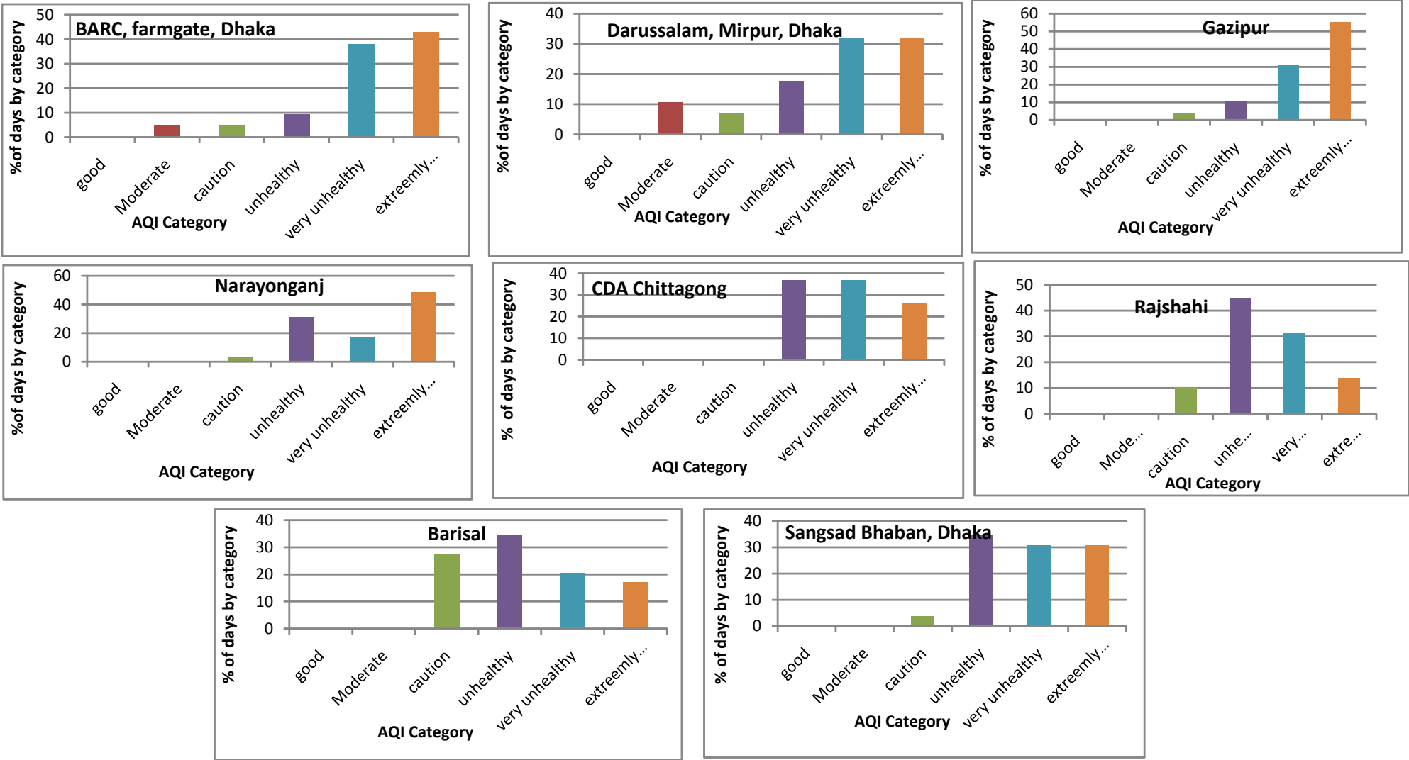
Figure 5: Monthly Summary of AQI for month of February, 2016
