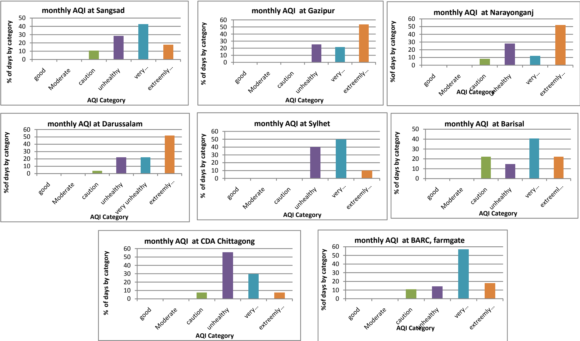
Figure 5: Monthly Summary of AQI for month of February, 2015
