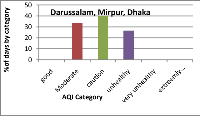
Figure 5: Monthly Summary of AQI for month of September, 2015
