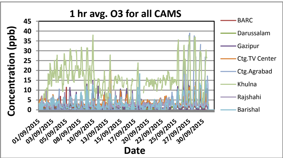
FIGURE 3: TIME SERIES OF ALL PARAMETERS (SO 2 , NO x AND O 3 ) MEASURED IN ALL CAMS DURING SEPTEMBER, 2015
