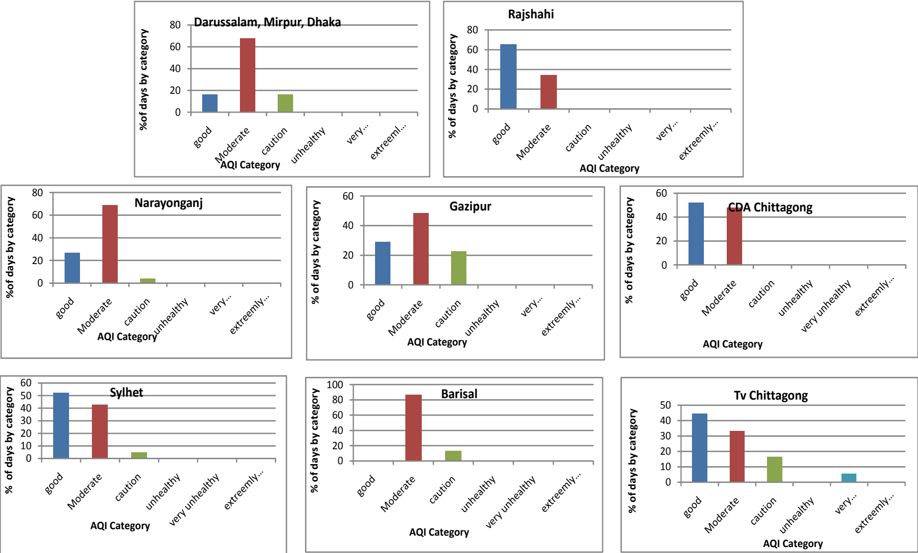
Figure 5: Monthly Summary of AQI for month of August, 2015
